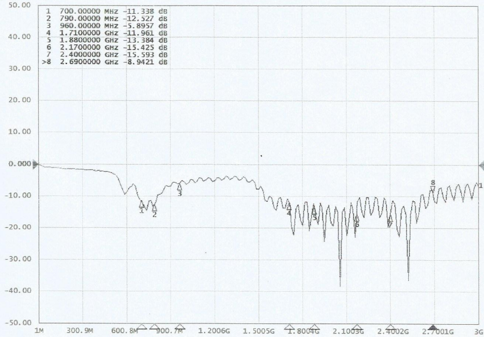
Fig 1 S11 Log Mag 10.00dB/ Ref 0.000dB [ro]
