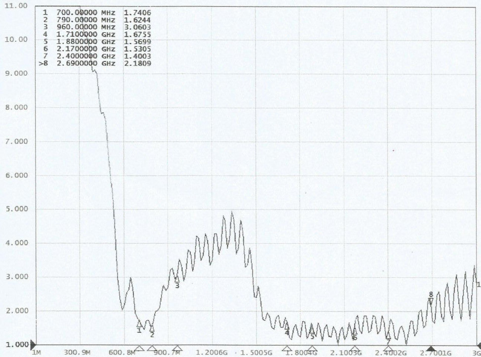
Fig 2 S11 SWR 1.000/ Ref 1.000 [RO]
