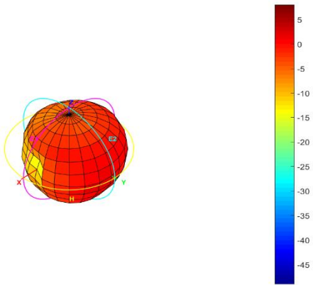
Total_3D_Side View 1_2.6GHz
