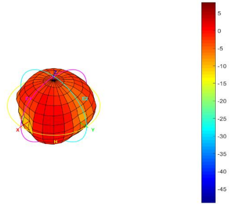
Total_3D_Side View 1_2.17GHz
