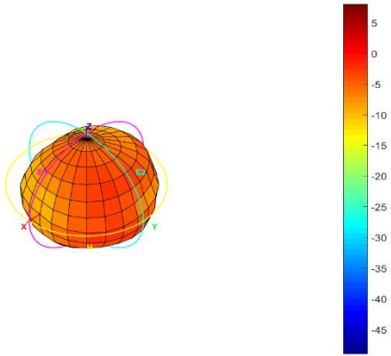
Total_3D_Side View 1_1.88GHz
