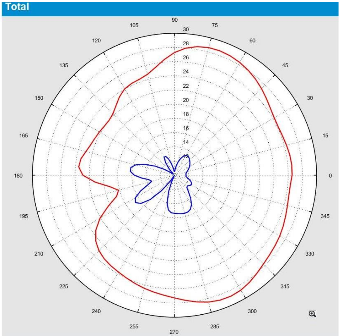
Total_Efficiency (%)
