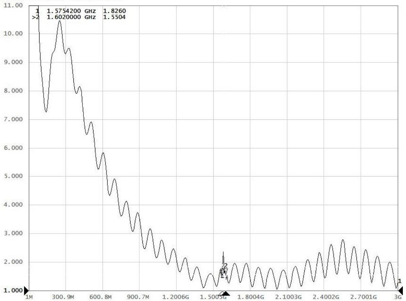
Tr1 S11 SWR 1.000/ Ref 1.000 [R0]
