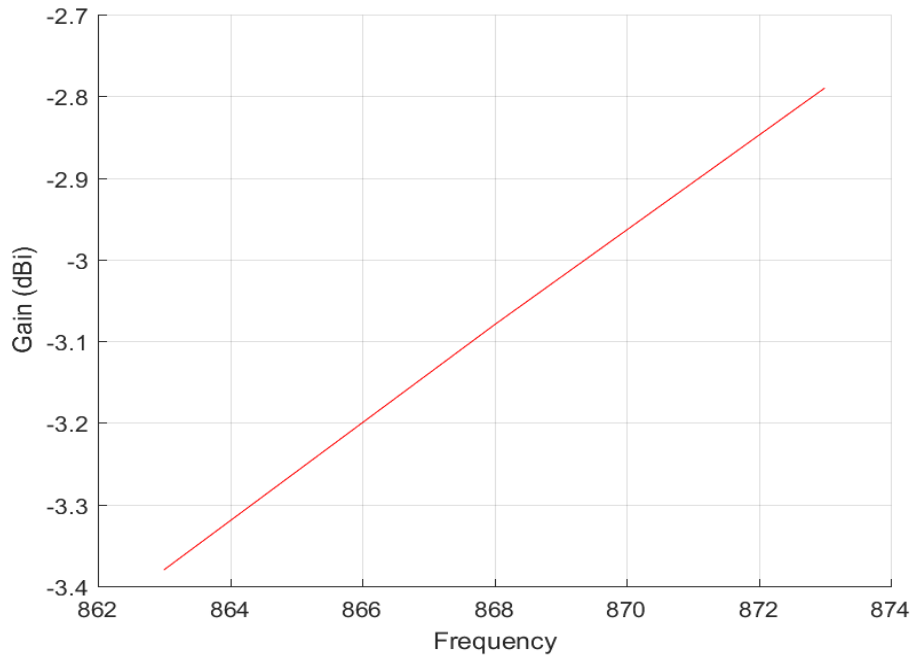
Total_3D_Side View 1_863MHz
