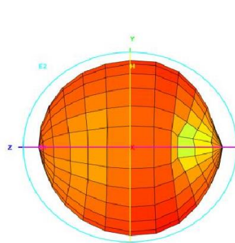
Total_3D_Left View_690MHz
