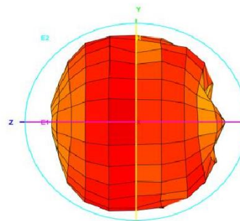
Total_3D_Top View_2.6GHz
