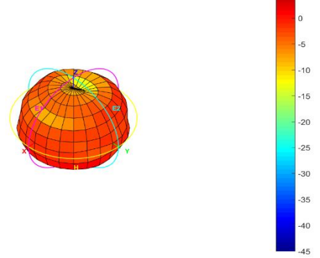
Total_3D_Front View_1.88GHz
