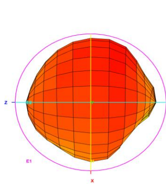
Total_3D_Top View_690MHz
