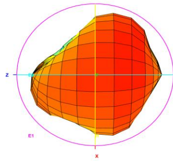
Total_3D_Left View_824MHz
