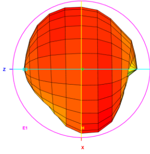
Total_3D_Left View_859MHz
