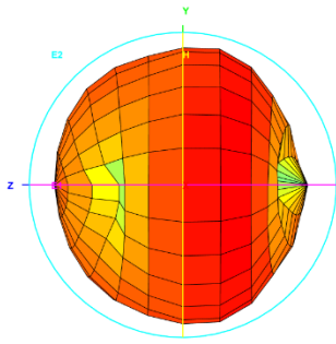
Total_3D_Top View_869MHz
