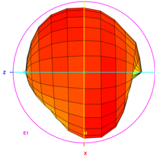
Total_3D_Left View_869MHz
