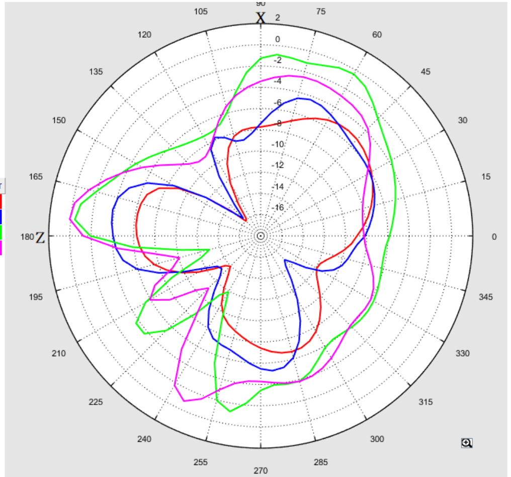
Total_Efficiency (%)
