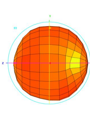
Total_3D_Left View_824MHz
