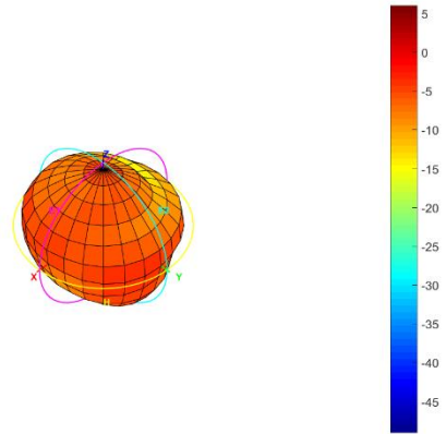
Total_3D_Front View_1.71GHz
