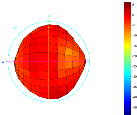
Total_3D_Left View_1.71GHz
