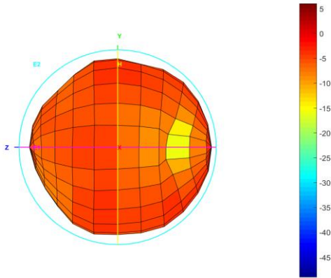
Total_3D_Top View_1.71GHz
