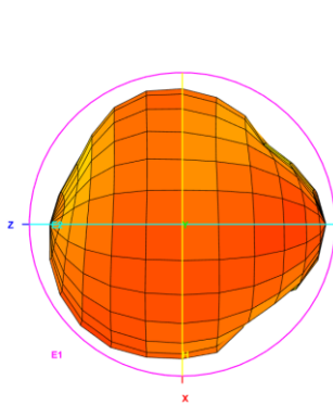
Total_3D_Top View_824MHz
