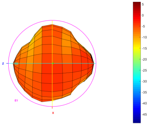
Total_3D_Left View_960MHz
