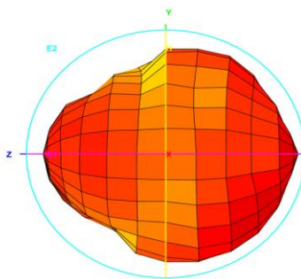
Total_3D_Left View_1.8GHz
