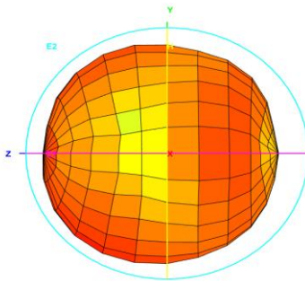
Total_3D_Left View_700MHz
