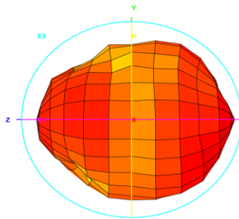
Total_3D_Left View_1.9GHz
