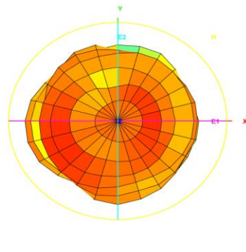
Total_3D_Top View_2.7GHz
