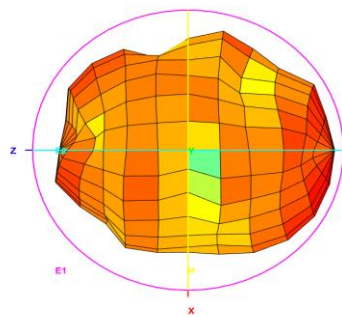
Total_3D_Side View_1_2.1GHz
