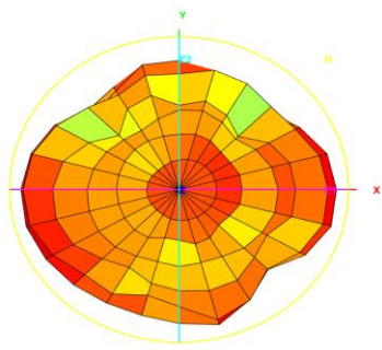
Total_3D_Front View_2.7GHz
