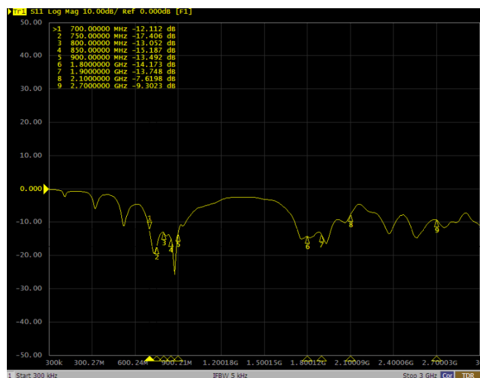
Test Data(Return Loss & VSWR)
