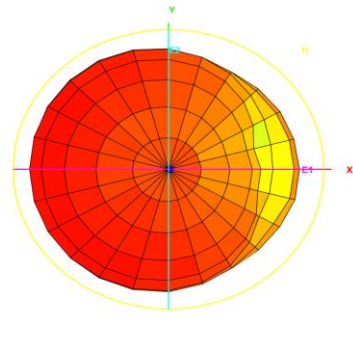
Total_3D_Side View 1_700MHz
