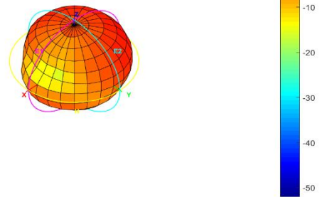
Total_3D_Front View_750MHz
