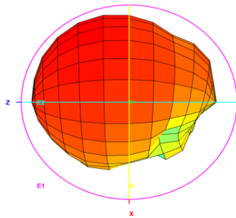
Total_3D_Left View_850MHz
