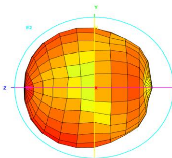
Total_3D_Left View_750MHz
