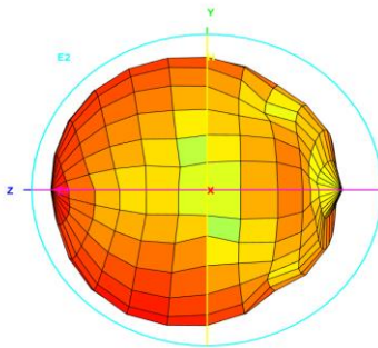
Total_3D_Left View_800MHz
