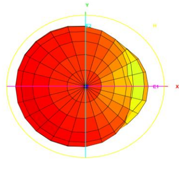
Total_3D_Side View 1_750MHz
