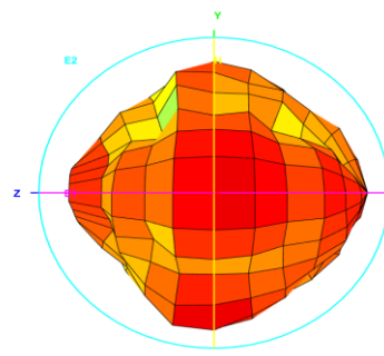
Total_3D_Left View_2.7GHz
