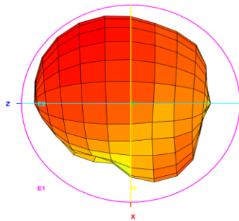
Total_3D_Left View_750MHz
