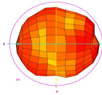
Total_3D_Left View_1.9GHz
