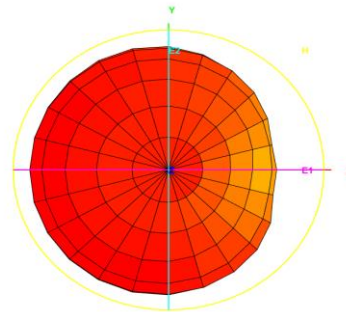
Total_3D_Side View 1_850MHz
